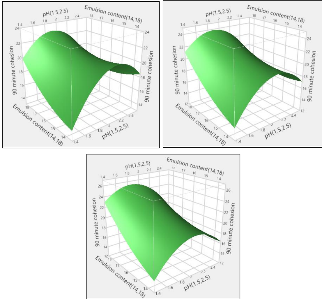
Figure 30. Surface response plots for cohesion development at 90 minutes at 4% water content (top left), 6% water content (top right) and 8% water content (bottom)
