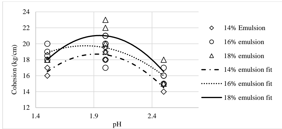
Figure 24. Cohesion vs. pH at 60 minutes
